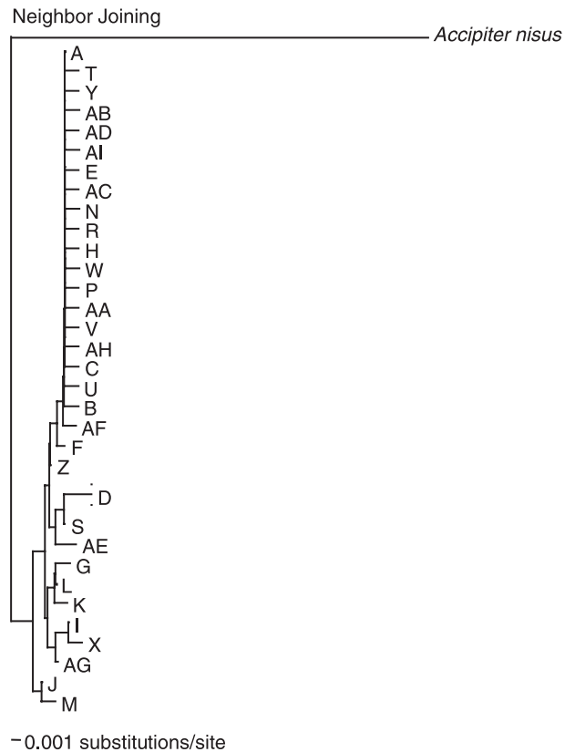
Fig. 2 Neighbour-joining tree from Tamura-Nei distances of control region haplotypes for Accipiter velox sampled in North America with Accipiter nissus as the outgroup (Tamura & Nei 1993).
